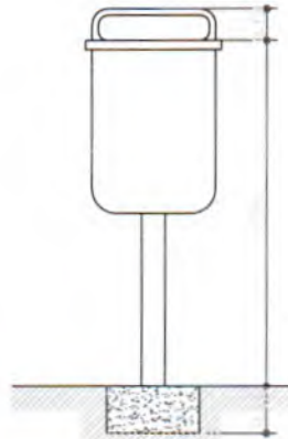
VISTA FRONTAL
